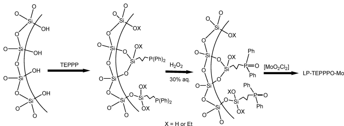
Scheme 1. Preparation of LP-TEPPPO-Mo by using the T-method.
