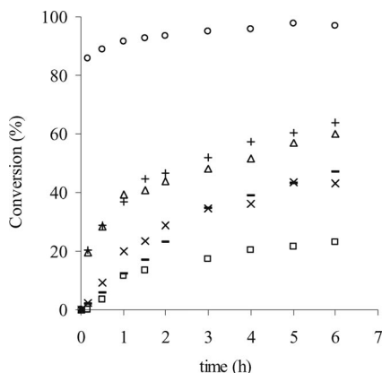
Figure 1. Reaction of cis -cyclooctene with t BuOOH at 55 °C without co-solvent in the presence of complex 1 (○), LP-TEPPPO (□), LP-TEPPPO-Mo [run 1 (+); run 2 (–)] or using the complex 1 /[BMPy][BF 4 ] liquid–liquid biphasic system [run 1 (Δ); run 2 (×)].
